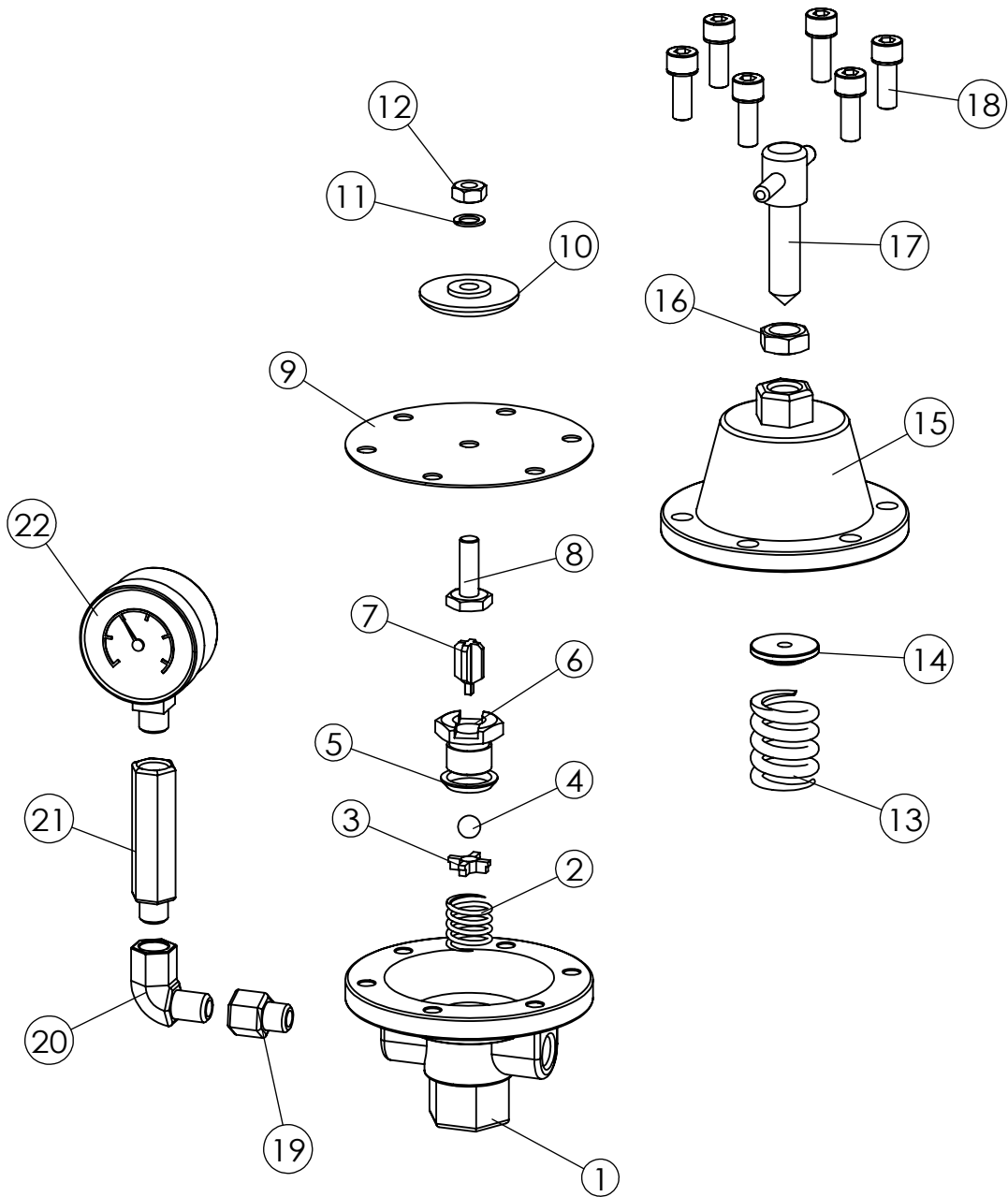
DS-A01P Dissolution Drawing
